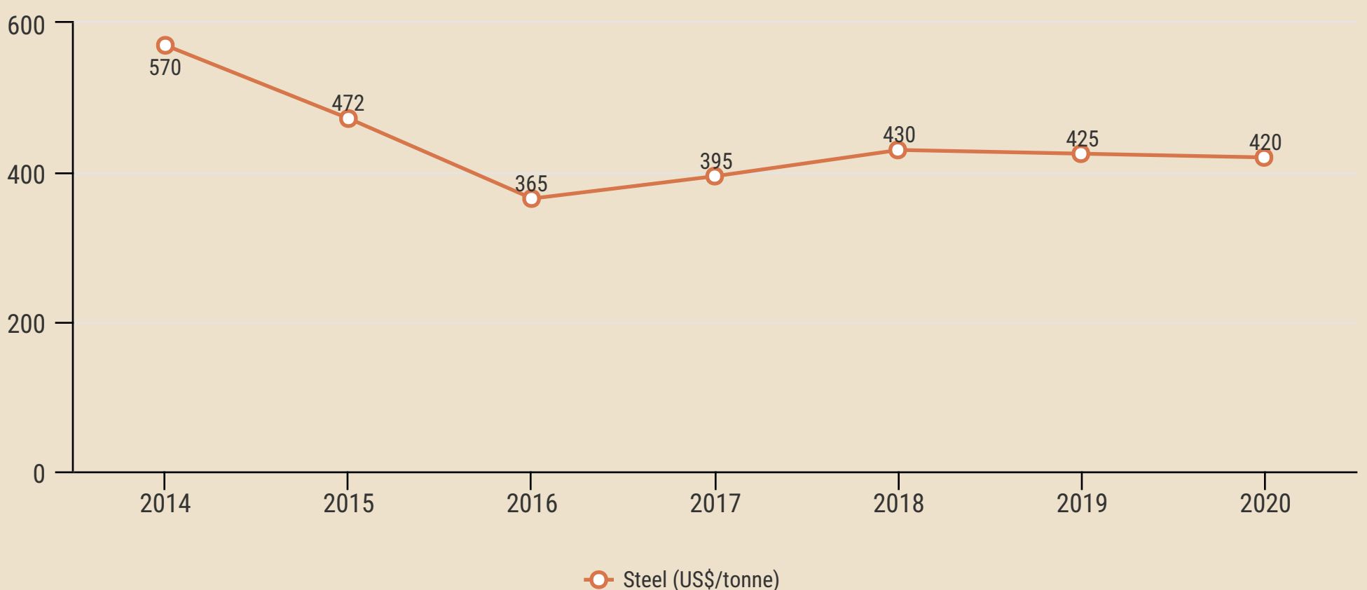
Price of Steel 2014-2020
